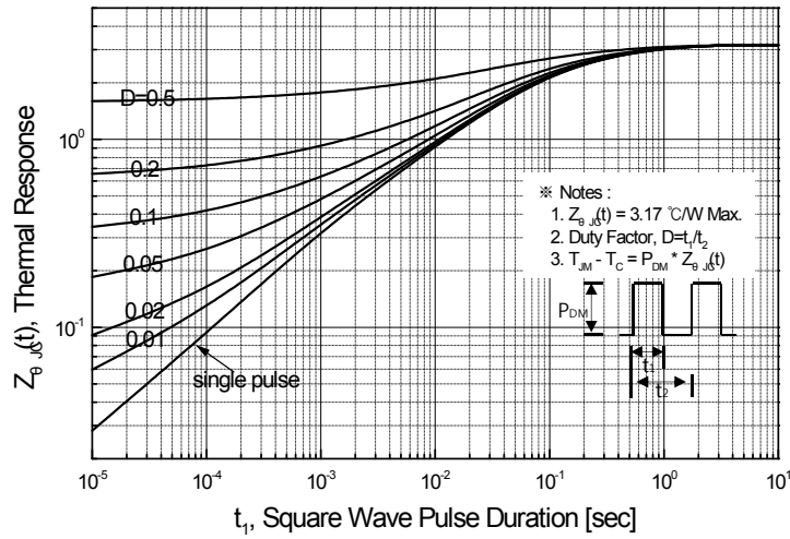
Figure 11-2. Transient Thermal Response Curve for SLF10N60C
