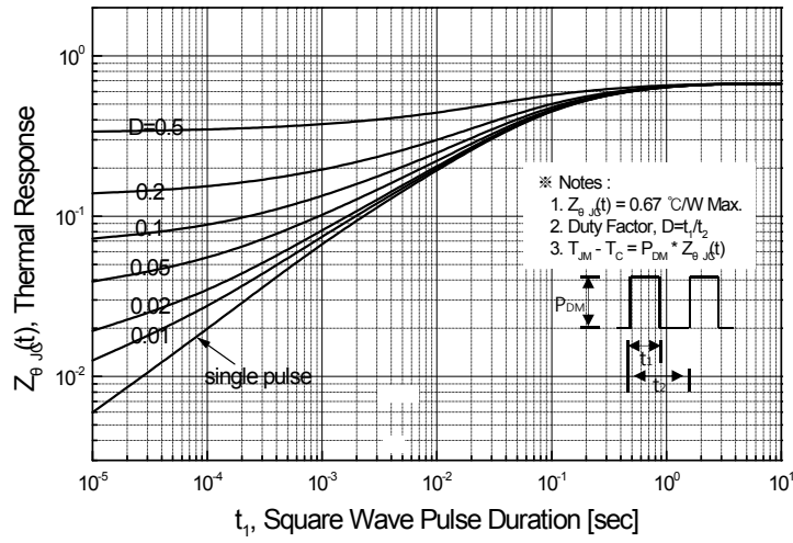
Figure 11-1. Transient Thermal Response Curve for SLP10N60C
