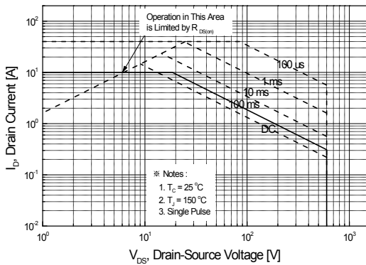
Figure 9-1. Maximum Safe Operating Area for SLP10N60C
