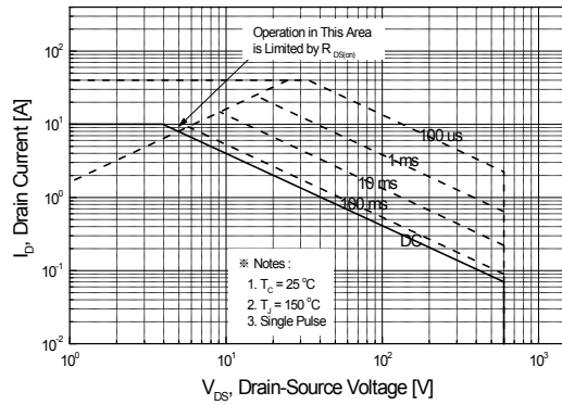
Figure 9-2. Maximum Safe Operating Area for SLF10N60C
