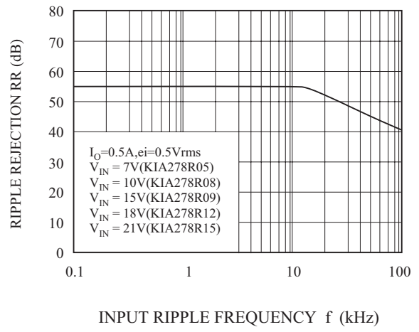
Fig. 10-1 f - RR
