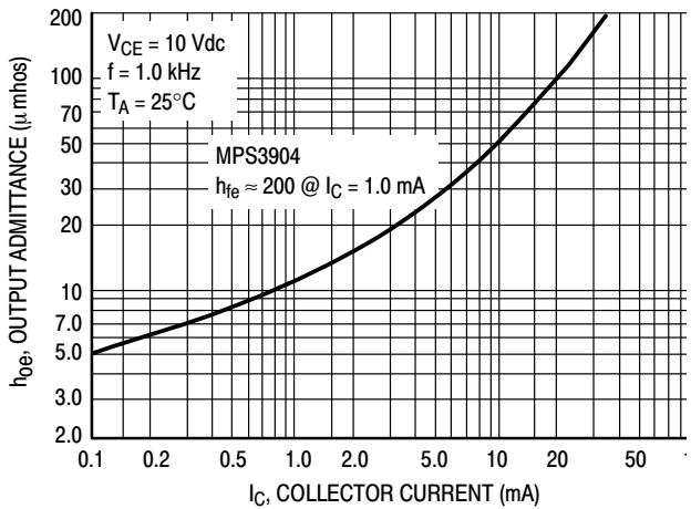
Figure 18. Output Admittance
