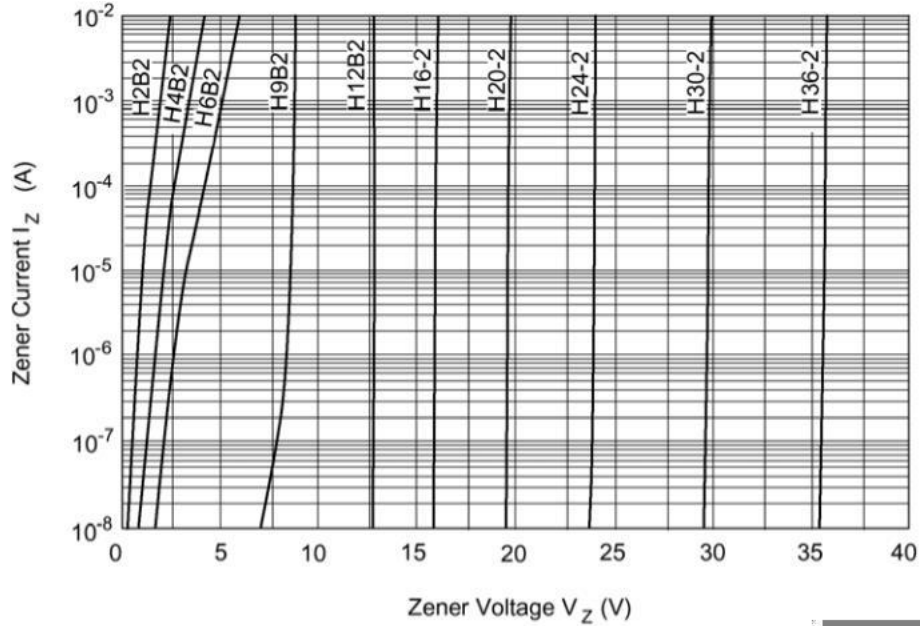
Figure 1. Zener current vs. zener voltage
