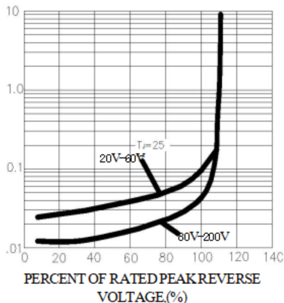
FIG.4-TYPICAL REVERSE CHARACTERISTICS
