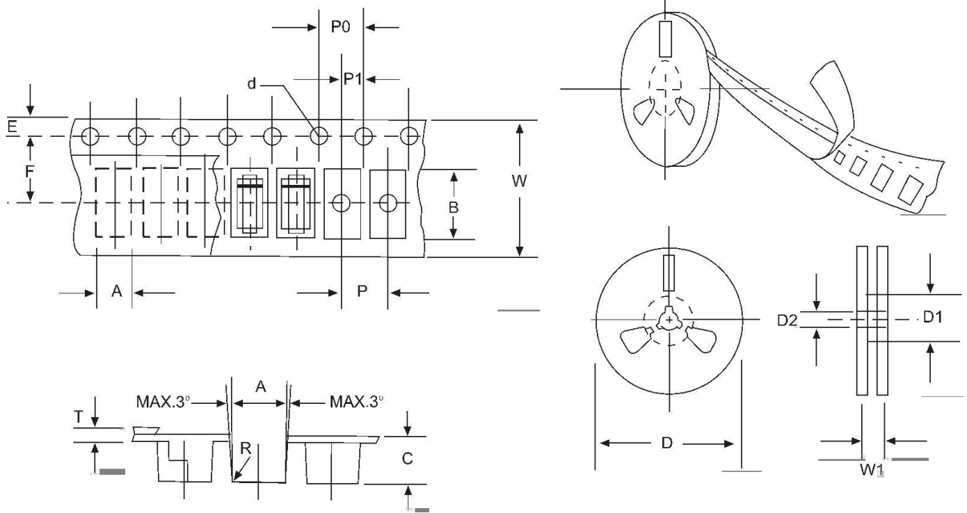
FIG: CONFIGURATION OF SURFACE MOUNTED DEVICE TAPING
