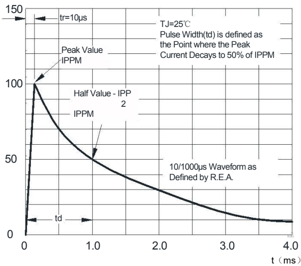
FIG3: Pulse Waveform
