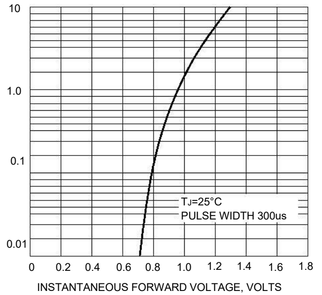
FIG.4-TYPICAL FORWARD CHARACTERISTICS
