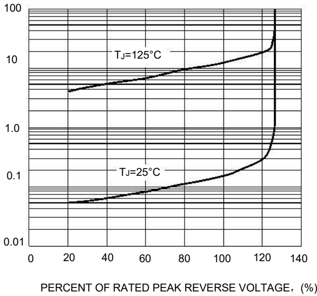
FIG.3-TYPICAL REVERSE CHARACTERISTICS
