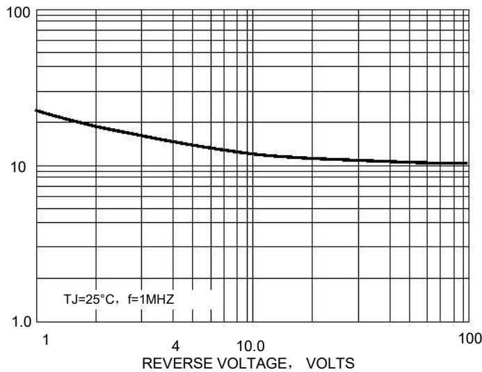
FIG.5-TYPICAL JUNCTION CAPACITANCE
