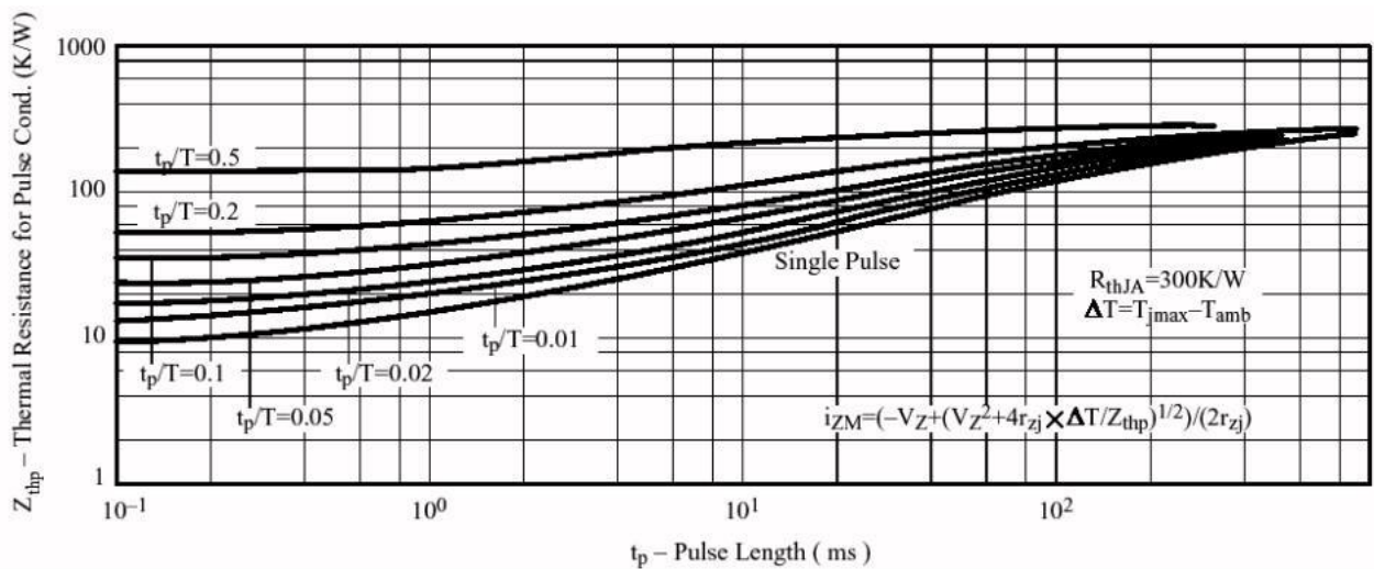
Figure 10. Thermal Response
