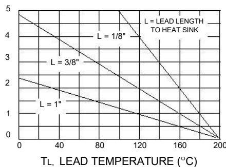
Fig. 1 Power Temperature Derating Curve
