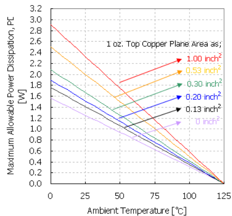
Maximum Allowable Power Dissipation, P_D vs. Ambient Temperature [TO263 Package]
